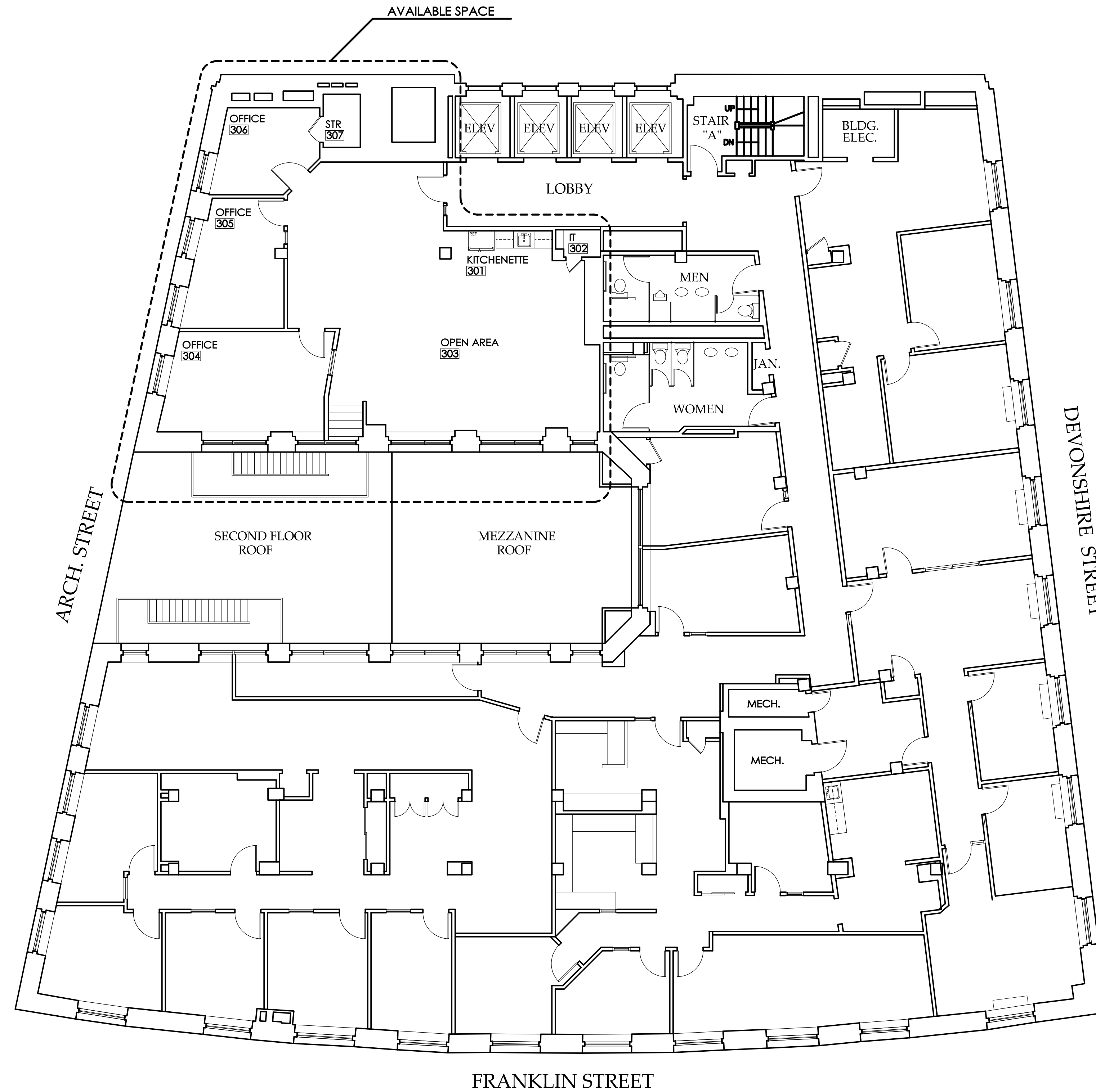
1 FLOOR PLAN 1/8" = 1'-0"
